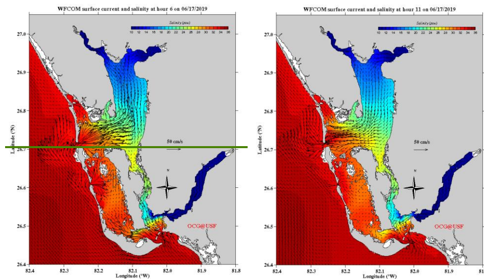
Figure 18. Screen capture of an online surface water model of the Charlotte Harbor area. Output shows hourly forecasts of surface currents and salinity for incoming and outgoing tides; generated from the West Florida Coastal Ocean Model | http://ocgweb.marine.usf.edu/Models/WFCOM/wfcom_index.html .
